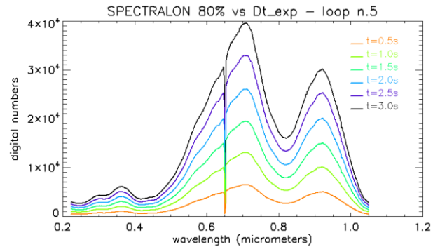
Fig. 26. Acquisitions at 7 different integration times. From orange to black curve, the t_{EXPO-VIS} increases linearly from 0.5 to 3.0 s.
