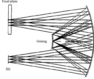
Fig.2. Offner spectrometer configuration adopted for the VIR instrument (De Sanctis et al., 2010).
