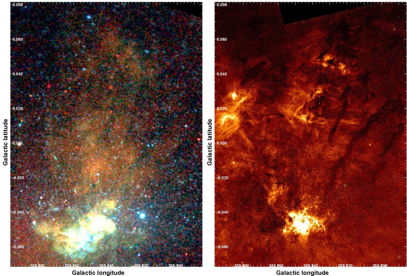
Figure 20. Left-hand panel: Chandra RGB image of the northern lobe. See Fig. 18 for more details. Right-hand panel Pa \alpha image of the northern lobe, tracing thermal, ionized gas (from Wang et al. 2010). Continuum emission from stars has been removed (Dong et al. 2011), so the only stars that appear are those that have strong Pa \alpha emission lines. Two Pa \alpha -emitting luminous stars located at l \sim 359^{\circ}935 , b \sim 0^{\circ}21 and l \sim 359^{\circ}925 , b \sim 0^{\circ}45 (Mauerhan et al. 2010; Dong, Wang & Morris 2012) are probably responsible for at least part of the ionization indicated by the Pa \alpha .
