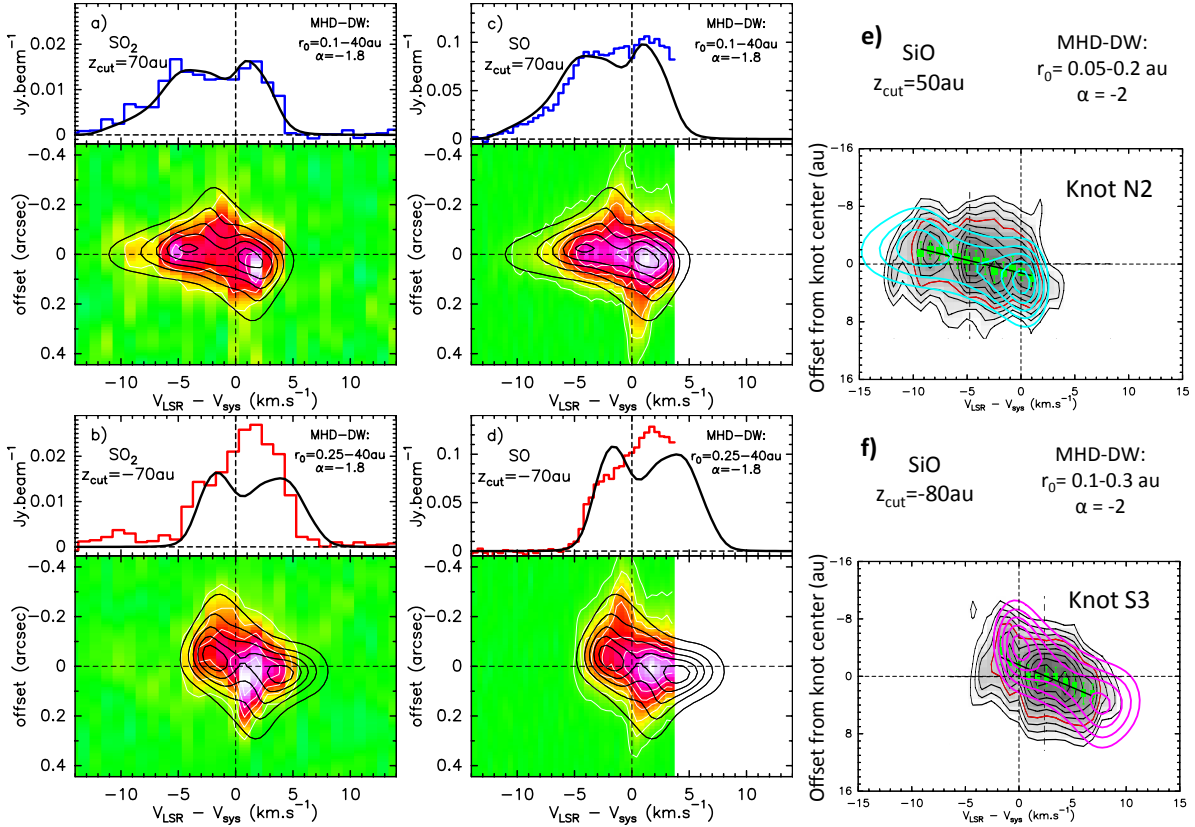
Fig. 2. Panels a–d : observed on-axis line profiles (histograms) and transverse PV diagrams (color map and white contours) of SO 2 ( left ) and SO ( middle ) at \pm 70 au across the northern blue jet ( top ) and the southern red jet ( bottom ). The red wing of SO falls outside our spectral set-up. A DW model fit, with \lambda = 5.5 and \mathcal{W} = 30 (see text), is overplotted in black for parameters denoted in each panel. Panels e–f : PV diagrams observed by Lee et al. (2017a) across the SiO knots N2 and S3 (grayscale and black/red contours). Their measured centroids are shown as green squares and fitted rotation gradient as a black line. The DW model is overplotted in cyan ( top ) or magenta ( bottom ) with parameters denoted above each panel.
