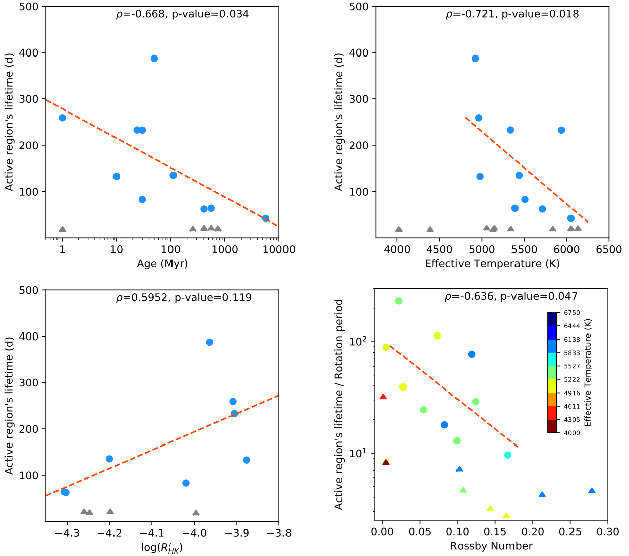
Fig. 10. Timescale of AR evolution derived from the ACF analysis of the TESS light curves as a function of stellar age ( top left ), effective temperature ( top right ), \log R'_{\text{HK}} value ( bottom left ), and Rossby number ( bottom right ). Stars with lower limits on the AR timescale are shown with triangles. A linear fit (dashed orange-red line) is shown to guide the eye.
