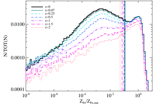
Figure 10. Distribution of the Fe abundance (w.r.t. solar values by ANGR89) for the hot-phase gas particles selected to reside within [0.75-1]R_{200} at z = 0 and tracked back in time, at various redshifts up to z = 2 . Vertical lines correspond to the MW value of each distribution.
