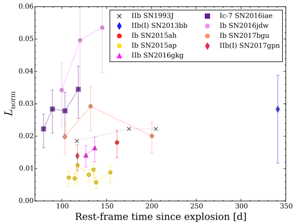
Figure 8. The normalised luminosity of the [O I] \lambda 6300,6363 line as derived from the nebular and near nebular spectra. Shown for reference is L_{\text{norm}} of type I Ib SN 1993J (Barbon et al. 1995; Richmond et al. 1996).
