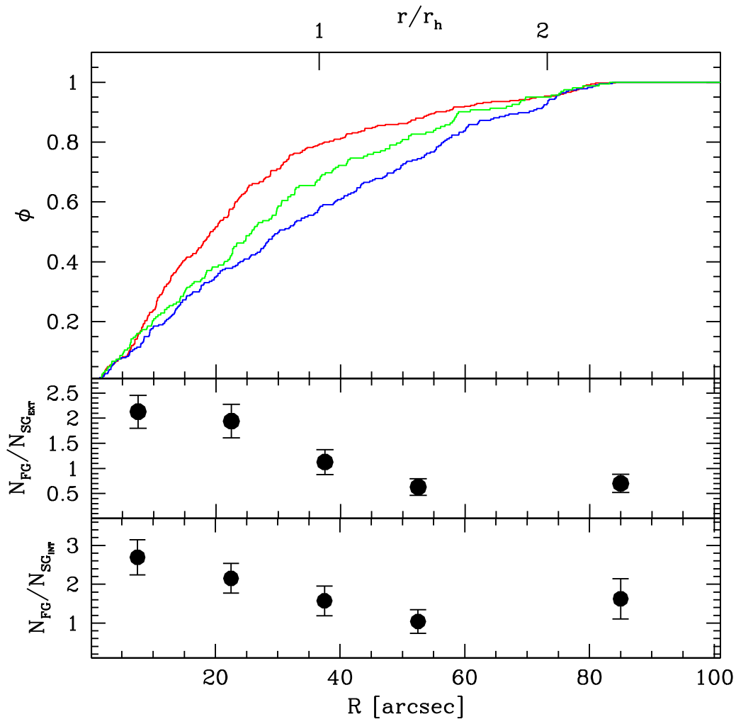
Figure 4. Upper panel: cumulative radial distribution of FG (red), SG_{INT} (green), and SG_{EXT} (blue) stars selected as detailed in Section 3. Lower panels: N_{FG}/N_{SG_{EXT}} and N_{FG}/N_{SG_{INT}} as a function of the distance from the cluster center.
