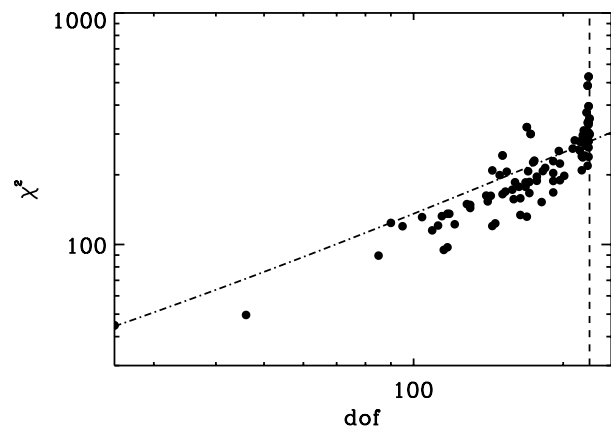
Fig. 2. Distribution of our best fit \chi^2 in function of the degree of freedom (dof) of each observation of our sample. The dot-dashed curve indicates the \chi^2 value corresponding to a 99% null hypothesis probability for the corresponding dof value. The vertical dashed line represents the 226 dof limit of our sample.
