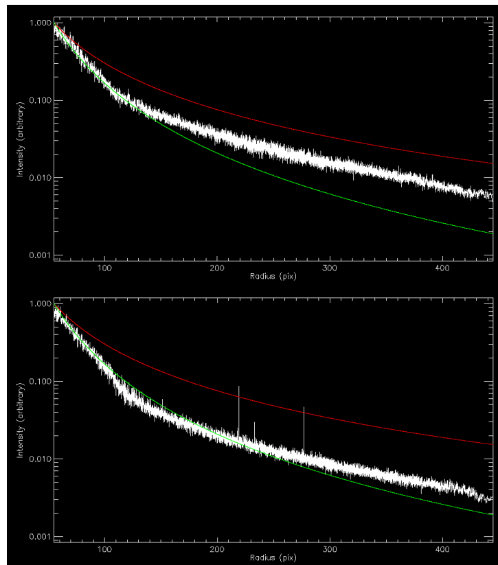
Figure 7: Radial profiles of the PSF wings outside the occultation mask without VPH (top) and with VPH at first order (bottom). The red and green lines are respectively the rescaled r^{-2} and r^{-3} behavior. The two profiles are very similar, confirming that there is no evidence of light diffusion to the PSF wings due to the VPH disperser.
