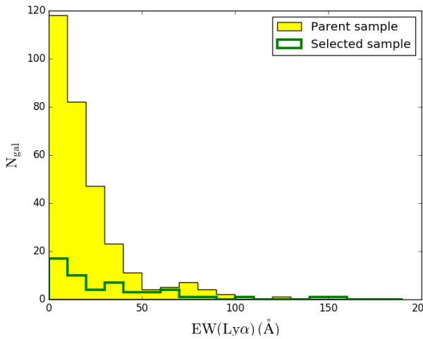
Fig. 6. Ly \alpha EW distributions for the sources in the parent sample (yellow histogram) and those in the selected sample (green empty histogram).
