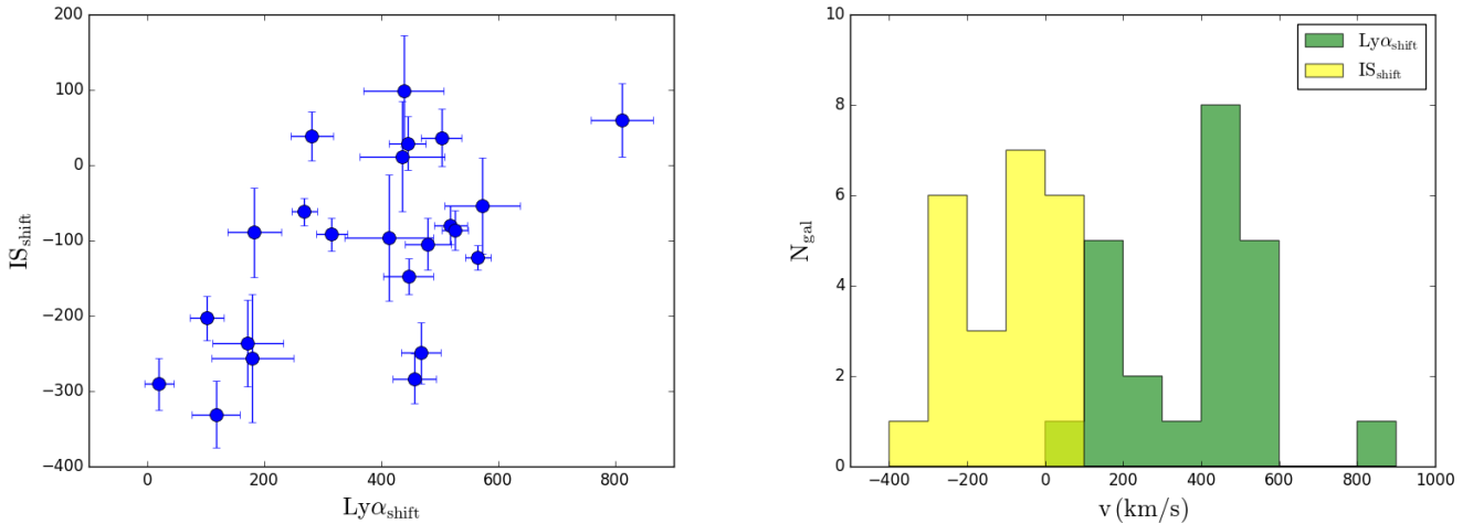
Fig. 10. Left panel: anticorrelation between the velocity of the main peak of the \text{Ly}\alpha profile with respect to the systemic redshift and the IS velocity shift. Right panel: histogram of the measured (centroid) velocities of interstellar absorption lines in yellow and \text{Ly}\alpha emission in green with respect to the galaxy systemic redshift derived from the centroid of either the \text{CIII}\lambda 1909 \text{ \AA} or the \text{HeII}\lambda 1640 \text{ \AA} emission lines. The yellow sample contains only the 26 objects for which we were able to give a precise measure of the IS velocity shifts, and the green sample contains the 46 spectra where we were able to estimate the \text{Ly}\alpha peak shift.
