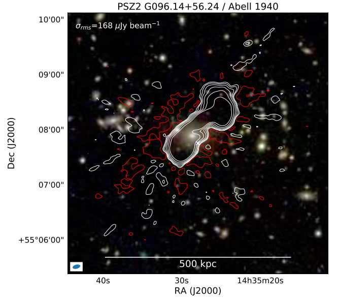
Fig. A.5. PSZ2 G096.14+56.24, Abell 1940. Optical image with robust -0.5 image radio contours. For more details, see the caption of Fig. 5.
