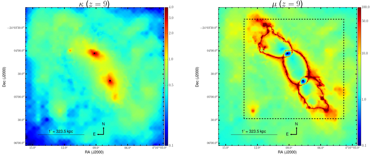
FIG. 5.— Left - Convergence ( \kappa ) map of MACSJ0416 produced by our lens model for a source at z_s = 9 . The convergence map reveals two primary total mass density peaks, centered approximately at the location of the two BCGs, which are marked by the two black points. Right - Flux magnification ( \mu ) map of MACSJ0416 produced by our lens model for a source at z = 9 . The approximate location of the critical curve, the curve along which magnification is maximized, can be seen. The dotted black square outlines the common area over which magnification maps were produced by all collaborative HFF modeling teams (see 5.1; Figure 6). Both the convergence and the magnification maps reveal a highly elliptical total mass distribution, as found by several other authors (e.g. Zitrin et al. 2013; Jauzac et al. 2014). Both maps cover the same 3.0 \times 3.0 \text{ arcmin}^2 footprint. The two black points on each map mark the centers of the two BCGs determined from the F105W image. Note that the colorbar is log-scale.
