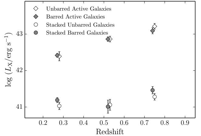
Figure 7. Average X-ray luminosities of barred (filled symbols) and unbarred (empty symbols) galaxies in three redshift bins for X-ray-detected active galaxies (diamonds) and undetected stacked galaxies (circles).
