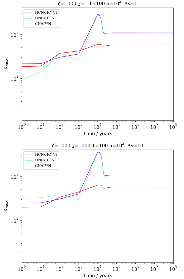
Figure 1. Plots showing the cases with significant ^{14}\text{N}/^{15}\text{N} increase, i.e. a fractionation decrease. In the title bar \zeta is in units of \zeta_0 , \chi in units of Draine, the temperature in units of Kelvins, the gas density in units of \text{cm}^{-3} , and the A_V is in magnitudes.
