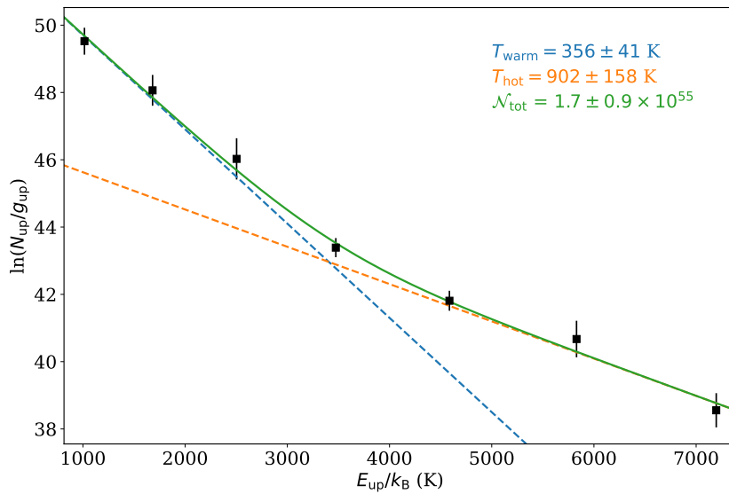
Fig. D.2. Rotational diagram of \text{H}_2 derived from the MIRI-MRS data. The black data points indicate the measured fluxes that are corrected for extinction (see Table. D.1). The best-fit two-component model is presented as the solid green line, and the two individual components are shown as the dashed blue (warm) and orange (hot) lines. The best-fit parameters are displayed in the top right.
