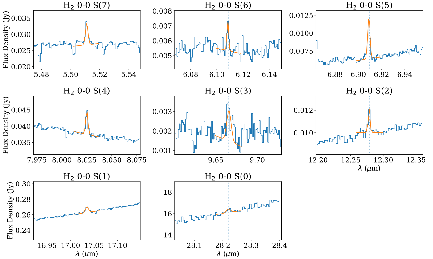
Fig. D.1. Observed MIRI-MRS spectrum (blue) centered around \text{H}_2 \nu = 0 pure rotational lines from the S(7) line in the top-left panel to the S(0) line in the bottom-middle panel. The best-fit Gaussian model is presented in orange in each panel. All presented lines are considered detected except for the S(0) line since the flux is similar to that of several strong residual fringes located in the vicinity of the S(0) line.
