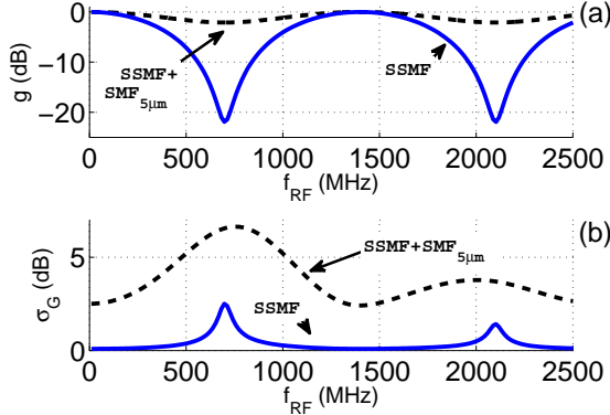
Fig. 1. Comparison of simulated results for a transmission link with SSMF length L_1 = 300 m in case of presence and in case of absence of SMF_{5\mu m} patch between SSMF and PD. The bandwidth improvement due to the SMF_{5\mu m} employment can be noticed in (a) while the increase of the standard deviation \sigma_G of the fluctuations of G due to modal noise is shown in (b). The parameters values utilized in the simulation program are: m_I = 0.375 , A_1^2 = 0.55 , A_2^2 = 0.45 , a_{11}^2 = 0.9 , a_{12}^2 = 0.065 , b_{11} = 0.985 , b_{22} = 0.985 , b_{12} = 0.015 .
