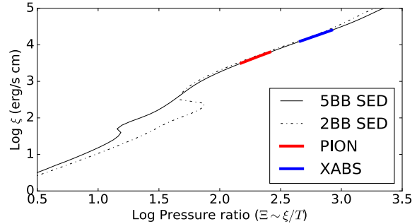
Figure A3. SED (top panel) and thermal-stability curve (bottom panel) computed for the time-averaged spectrum of NGC 247 ULX-1. The baseline SED (solid black line) consists of five unabsorbed blackbody models that account for emission in the optical, UV and X-ray bands. An alternative, simpler SED model uses just the X-ray two-blackbody model (dashed-dotted line).
