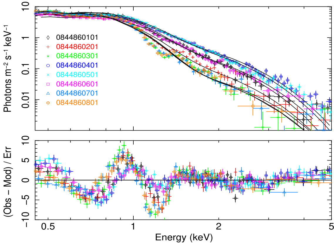
Figure 3. XMM- Newton EPIC-pn spectra of NGC 247 ULX-1. The top panel shows the pn spectra of the individual observations with overlaid the 2-blackbody continuum models. The bottom panel shows the corresponding residuals. Both the emission feature below 1 keV and the absorption feature above 1 keV vary in centroid and strength according to the continuum flux and shape. This is qualitatively similar to the intermediate-hard source NGC 1313 ULX-1 and the soft source NGC 55 ULX-1 (Middleton et al. 2015b; Pinto et al. 2017).
