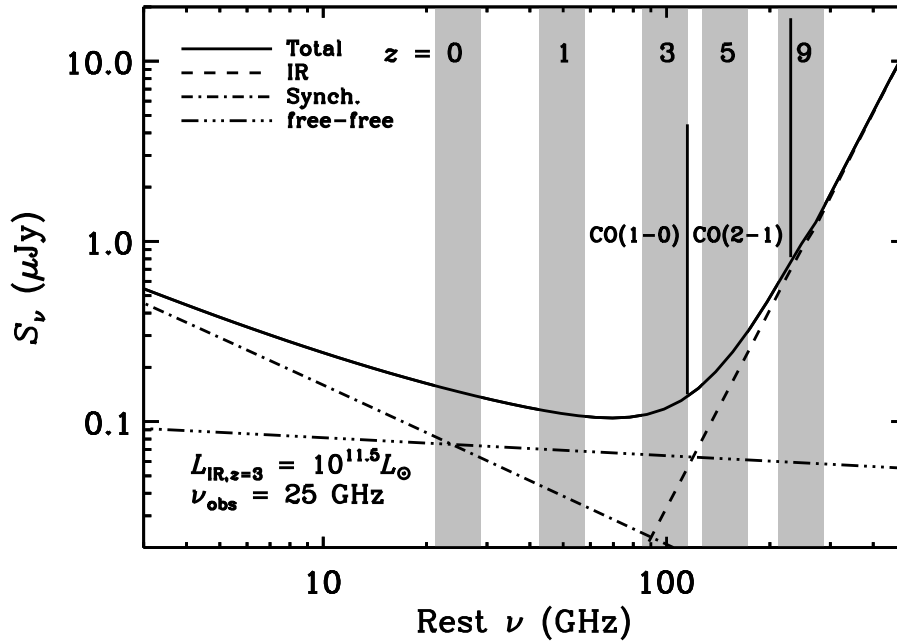
Figure 1: A rest frame model radio-to-infrared galaxy spectrum having an IR ( 8\text{--}1000\mu\text{m} ) luminosity of L_{\text{IR}} = 10^{11.5} L_{\odot} at redshift 3. The shaded regions indicate where a 25 GHz observation (see §3), having 30% bandwidth in the observed frame, would redshift for z = 0, 1, 3, 5, and 9 . Individual emission components (free-free, synchrotron, and thermal dust) are shown, indicating that at this frequency range between 30 and 100 GHz (in the rest frame) is most sensitive to free-free emission, making this spectral window extremely robust for accurately measuring the star formation rates of high-redshift galaxies. Additionally shown are CO ( J = 1 \rightarrow 0 ) and CO ( J = 2 \rightarrow 1 ) spectral lines having a line-to-IR flux ratio of M 82 and 1000 \text{ km s}^{-1} widths. These lines, which are essential for accurately measuring the molecular gas content of galaxies as they trace the bulk of the cold molecular gas component, are accessible in the redshift range of z = 2.8 - 10.5 over the full 20 – 30 GHz spectral window.
