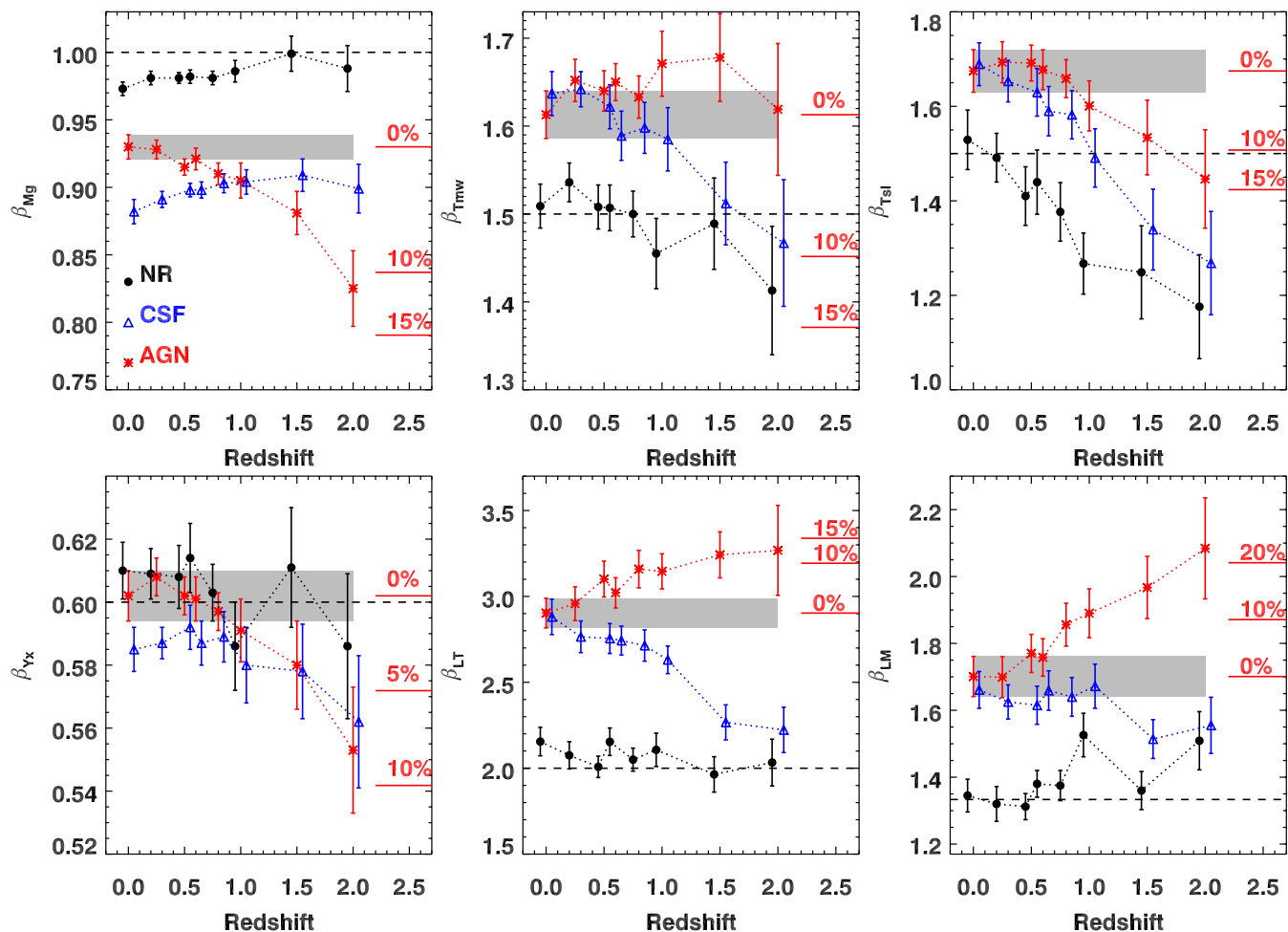
Figure 5. We show the slope value for M - M_g , M - T_{mw} , M - T_{sl} , M - Y_X , L - T_{sl} , and L - M shown from left to right, top to bottom, respectively, as a function of redshift. In each panel, the NR, CSF, and AGN runs are represented by the black circles, open blue triangles, and red asterisks. The dashed black lines represent the self-similar evolution of the slopes. The error bars represent 1\sigma of the \beta parameter. The grey shaded area shows its value at z = 0 for the AGN sample. In this run, we notice that the slopes at redshifts z < 1 agree within 1\sigma with the z = 0 value, while at higher redshifts they can significantly deviate. Some variations from the z = 0 value of the AGN sample are reported with red horizontal lines on the right part of the plots.
