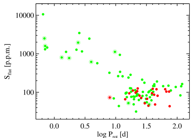
Figure 14. STD of the flattened light curve excluding the outliers, as in Fig. 6, shown here versus rotation period. Green symbols (period flag ‘Y’), red symbols (period flag ‘?’). The clear transition between fast and slowly rotating stars indicates that for fast rotators the origin of this ‘noise’ has an astrophysical component. Binaries are highlighted with annuli.
