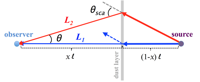
Figure 1. Geometry of the dust scattering by a single dust layer. \theta is the viewing angle. \theta_{\text{sca}} is the scattering angle. \ell is the absolute distance between the source and the observer. x is the fractional distance from the dust layer to the observer. L_1 and L_2 signify the two different light paths traveled by a LOS photon and a scattered photon in the halo.
