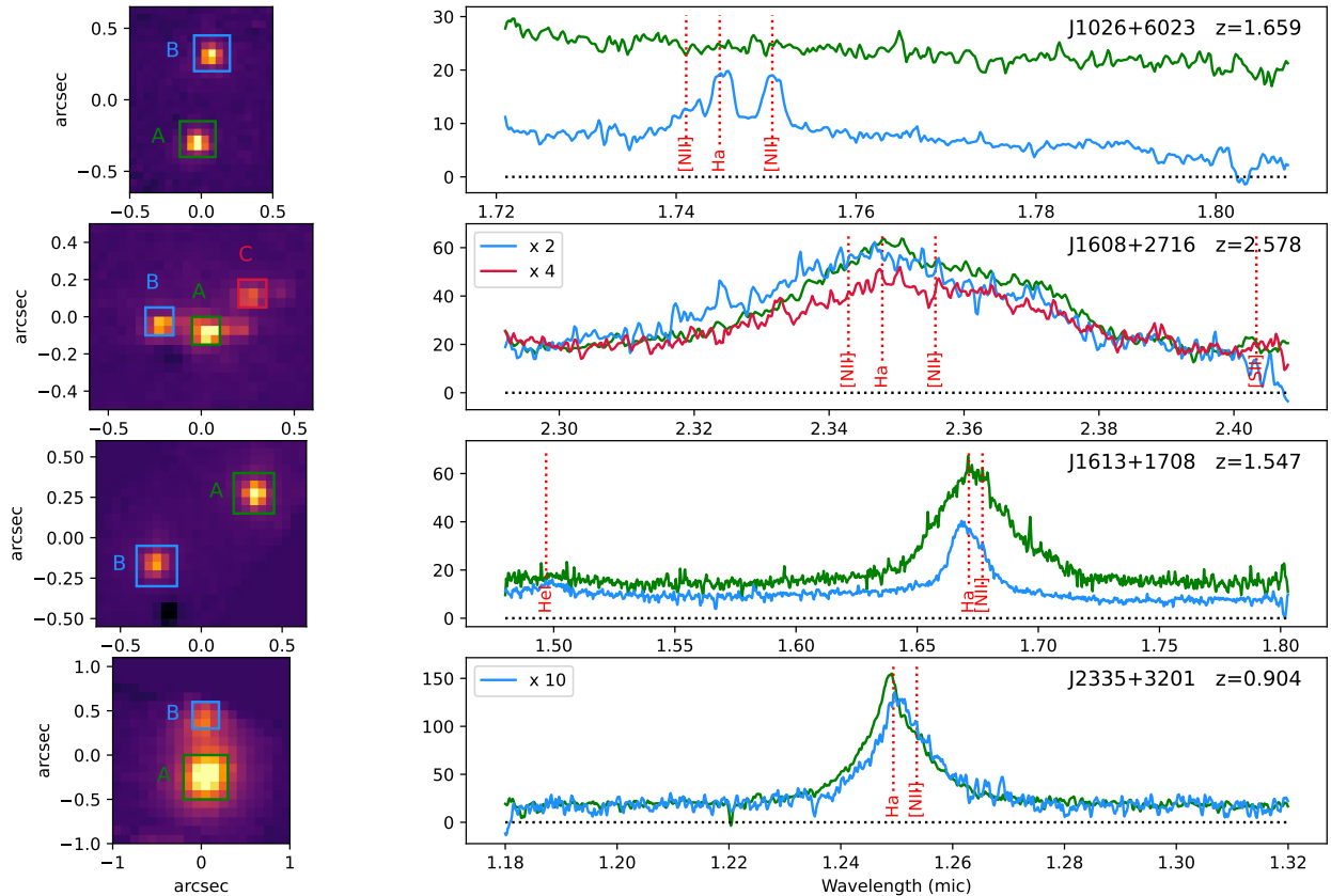
Fig. 1. H \alpha emission line maps (left) and spectra (right) of the systems observed with OSIRIS (the target name and redshift are reported in the right panels). The line maps are oriented with north being up and west to the right. The spectra shown in the right panels have been extracted over the squared apertures marked in the left panels (with the same color-coding). Each component of the systems is labeled as in Table 2. To optimize the visualization, some of the spectra have been multiplied by the factors indicated in the labels. Vertical dotted lines show the position of the main expected emission lines.
