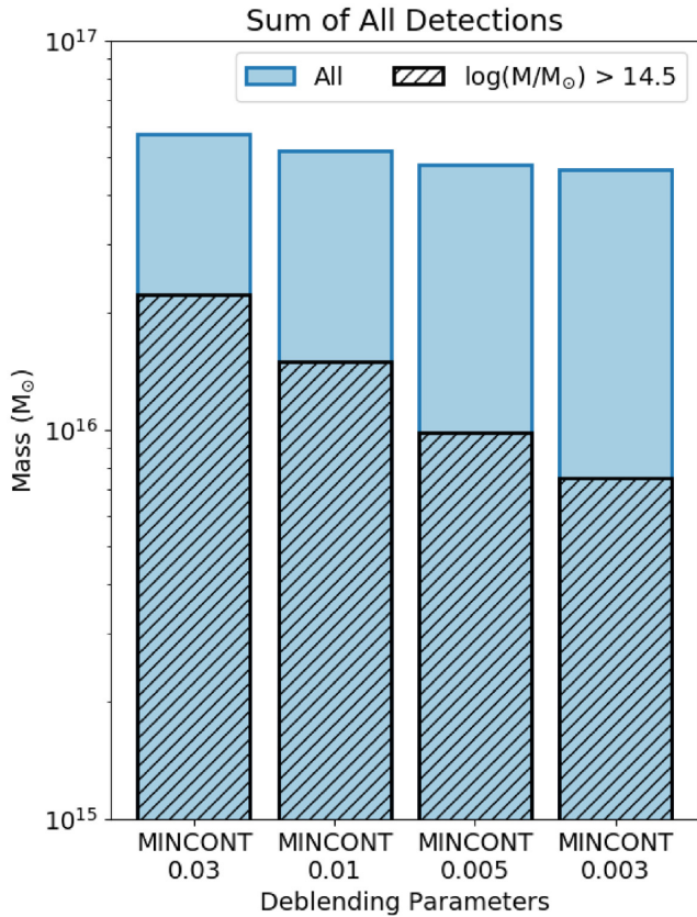
Figure 2. We plot the total mass of all overdensity candidates we find while varying the SExtractor debblending parameter DEBLEND_MINCONT . The debblending becomes finer for smaller values of DEBLEND_MINCONT . Following our expectations, finer debblending yields more low-mass overdensity candidates as more high-mass structures are broken up. Between the DEBLEND_MINCONT extremes plotted, the total mass decreases by 19 per cent, while the fraction of high-mass candidates drops by 66 per cent.
