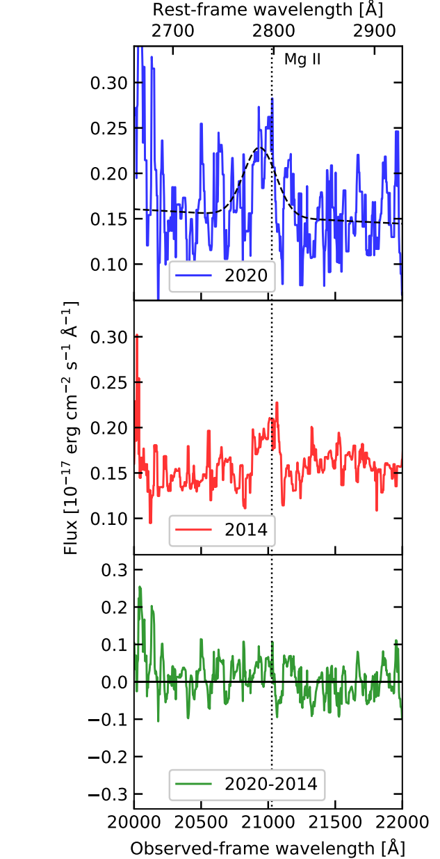
Fig. 7. Zoom-in of the spectral region of the 2020 ( top panel ) and 2014 ( middle panel ) spectra encompassing the Mg II emission line of PSO167–13. Bottom panel : difference between the two epochs. The dashed black line in the top panel marks the best fitting continuum plus single Gaussian model of the Mg II emission line.
