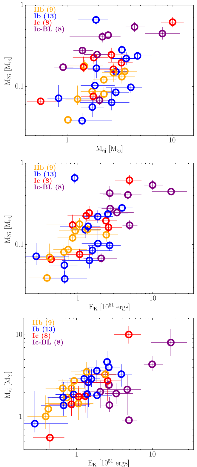
Figure 8. Derived explosion parameters ( M_{\text{Ni}} , M_{\text{ej}} and E_{\text{K}} ) of literature SE SNe are plotted against each other. Data are given in Table 5. SNe are colour-coded according to their type.
