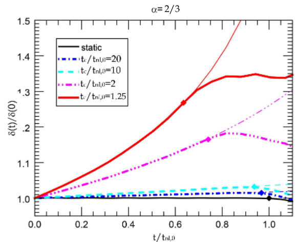
Figure e 3. Time evolution of the rms amplitude of density perturbations in an isothermal gas contracting isotropically with the scale factor of eq. (46) with \alpha = 2/3 (case of dynamical contraction) for various values of t_c (thick lines). Time is in units of t_{1,0} , the nonlinear time for the static model. diamond marks the position of t_1 given by eq. (47), and thin lines show the evolution of the amplitude in the WKB approximation. For t > t_1 shocks are formed and the waves dissipate.
