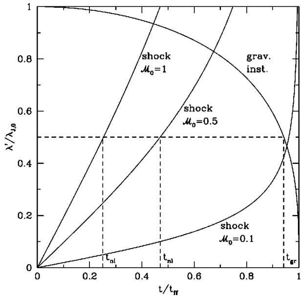
Figure e 2. During the collapse of a pressureless cloud, a linear perturbation with comoving wavelength \lambda' becomes nonlinear at a time t_1 (curves labelled “shock”) and gravitationally unstable at a time t_G (curve labelled “grav. inst.”). Wavelength is in units of the Jeans wavelength \lambda_{j,0} and time is in units of the cloud’s free-fall time t_{ff} . The non-linear time is shown for three values of the initial Mach number of the perturbations, \mathcal{M}_0 = 1 , \mathcal{M} = 0.5 and \mathcal{M}_0 = 0.1 . The case of \lambda' = 0.5\lambda_{j,0} is shown as an example: the nonlinear phase is reached before the gravitational instability, unless the perturbations have Mach number below \sim 0.1 .
