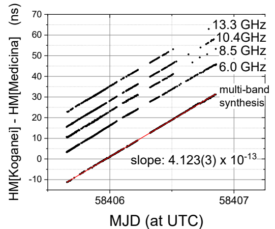
Fig. 2 Change of the time difference between two HMs in NICT(Koganei) and INAF(Medicina) using VLBI technique, where delays are measured in four frequency bands followed by multi-band analysis. The fractional frequency difference of two HMs is calculated from the slope.
