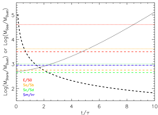
Fig. 8. Model predictions for M_{\text{Stars}}/M_{\text{Dust}} (dotted, black) and M_{\text{Gas}}/M_{\text{Dust}} (dashed black) ratios as a function of the SFR parameter t/\tau , using a value of \eta p = 2.0 \times 10^{-3} . The mean observed values of M_{\text{Stars}}/M_{\text{Dust}} (dotted) and M_{\text{Gas}}/M_{\text{Dust}} (dashed) for galaxies of different morphological types are indicated by the coloured lines.
