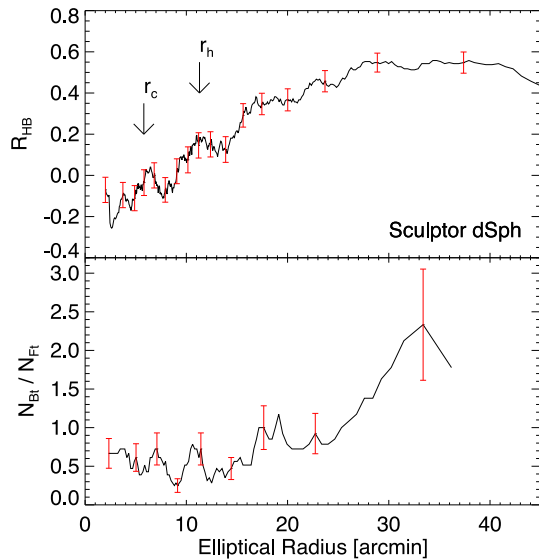
Figure 5. Top. The R_{\text{HB}} parameter as a function of the elliptical radius. The vertical arrows mark the core ( r_c = 5.8 arcmin, Mateo 1998) and half-light radius ( r_h = 11.3 arcmin, Irwin & Hatzidimitriou 1995). The vertical red lines display the errors on R_{\text{HB}} based on Monte Carlo simulations. The Bottom. Same as the top, but for the ratio between bright and faint RRLs in the full sample.
