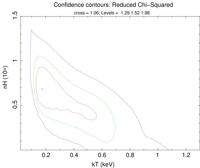
Figure 8. Contour plot of the temperature and absorption column parameters from a fit of an intrinsically absorbed MEKAL model to the Swift observation of 2017 July (assuming z = 0.0054 and a galactic column density nH = 2.0 \times 10^{21} \text{ cm}^{-2} ). The contours mark the 1\sigma , 2\sigma and 3\sigma errors.
