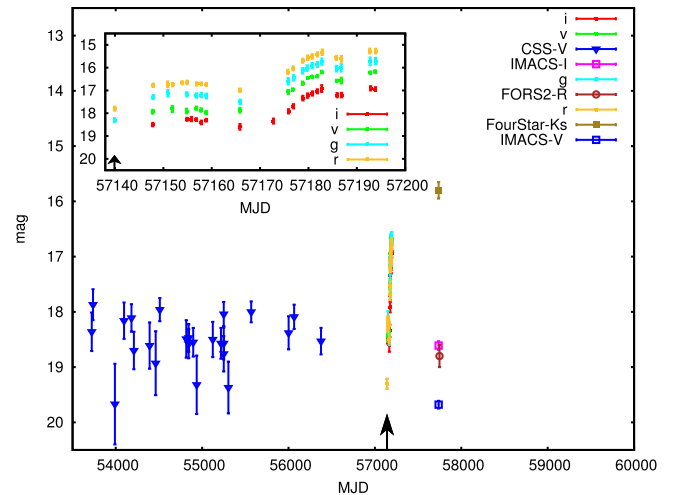
Figure 4. The multi-band light curve of the target, including the CSS data (filled triangles; see the text for details), is shown. The inset shows a zoom-in of the light curve (dots as taken directly from Childress et al. 2015) about the time of the SN event that occurred on 2015 April 27.9 UT (corresponding to MJD = 57139.9, as also indicated by the black arrow). From the i band to the r band we applied a recursive offset of 0.5 mag for each light curve shown in the inset. The data used to create this figure are available.
