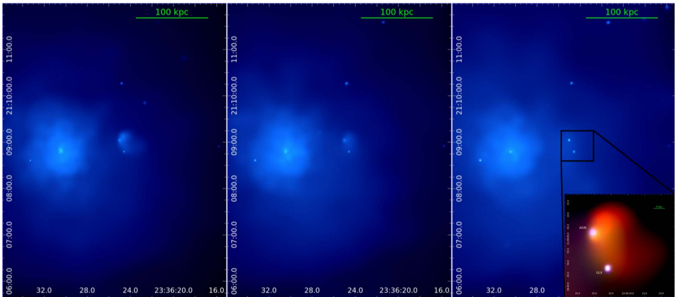
Figure 4. Cluster-scale images showing the three X-ray bands (soft 0.5–1.2 (left), medium 1.2–2.0 (middle), and hard 2.0–7.0 (right) keV) of the field of JW100, smoothed with smooth in CIAO. The inset in the right panel is an RGB (red = 0.5–1.2, green = 1.2–2.0, and blue = 2.0–7.0 keV) smoothed zoom on the galaxy where the two point sources (AGN and ULX candidate) are clearly visible.
