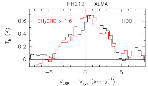
Fig. 3. Comparison between HDO(3 3,1 –4 2,2 ) (black line) and CH 3 CHO(18 0,18 –17 0,17 )A (red, multiplied by a factor of 1.6) as observed towards HH212–MM1 (in T_B , scale). The vertical dashed line defines the velocity with respect to V_{\text{sys}} = +1.7 km s ^{-1} (see footnote 2).
