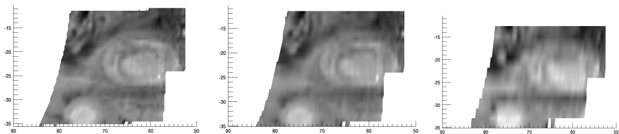
Figure 8 – The image of Figure 7 projected in System III planetocentric coordinates. In the three panels we show the image obtained by removing 2 (a), 4 (b) and 8 (c) lines every one from the original image, and linearly interpolating the surviving ones. This operation simulates the result achievable from 0.06, 0.13 and 0.25 of degree separation, respectively, between the consecutive slits of a future real observation of the JIRAM spectrometer.
