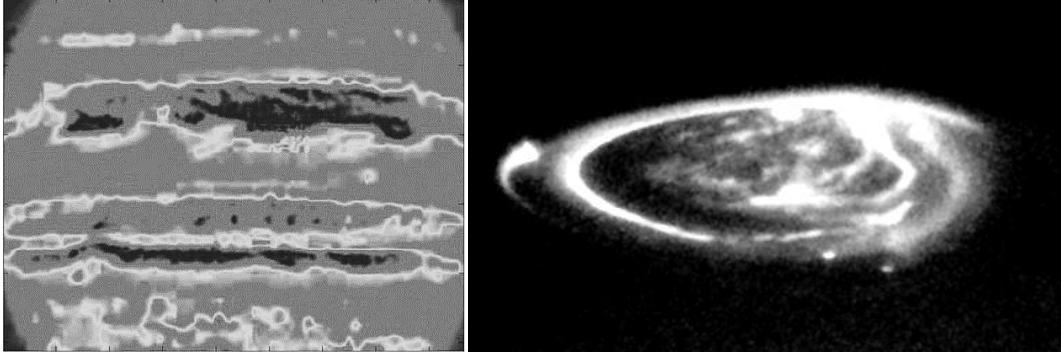
Figure 2 – Two sample pictures of Jupiter used to check the tolls for the noise reduction. Panel a: the planetary disk at 5 μm. Panel b: the North Pole aurora at UV wavelength.
