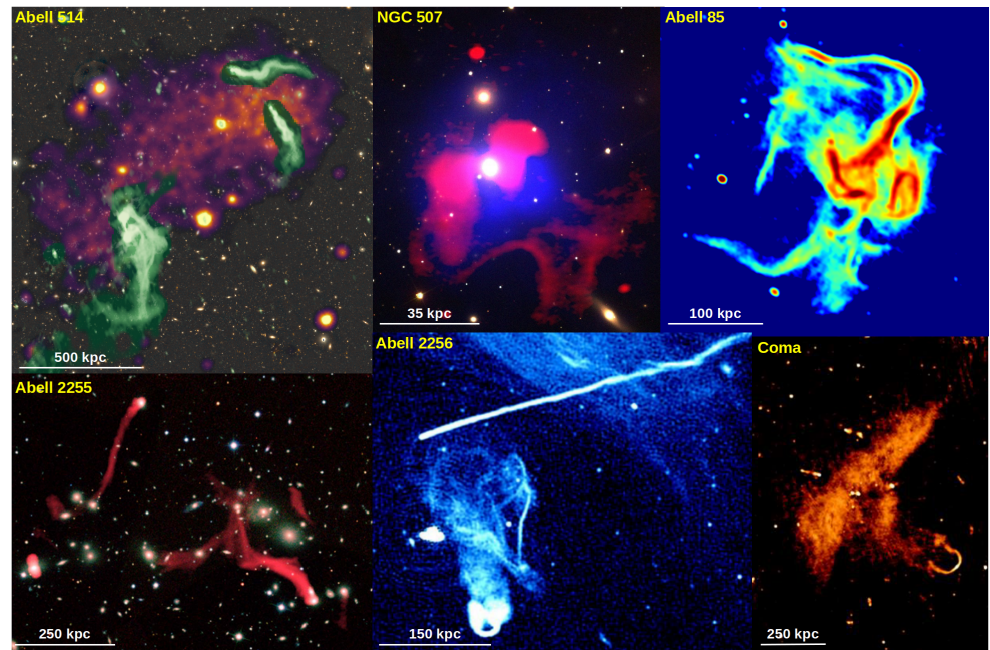
Figure 1. Examples of ongoing cosmic ray seeding and interaction between radio galaxies and thermal gas. From top left to bottom right: AGN with bended radio tails (green) due to the interaction with the X-ray gas (purple) in Abell 514 [37], radio plasma (red) transported by thermal gas (blue) sloshing motions in the NGC 507 group [19], the filamentary radio phoenix in Abell 85 [38], the complex system of filamentary tailed radio AGN (red) at the center of Abell 2255 [39], the radio phoenix and the long head-tail radio galaxy in Abell 2256 [40], a radio galaxy feeding the radio relic in the Coma cluster [41].
