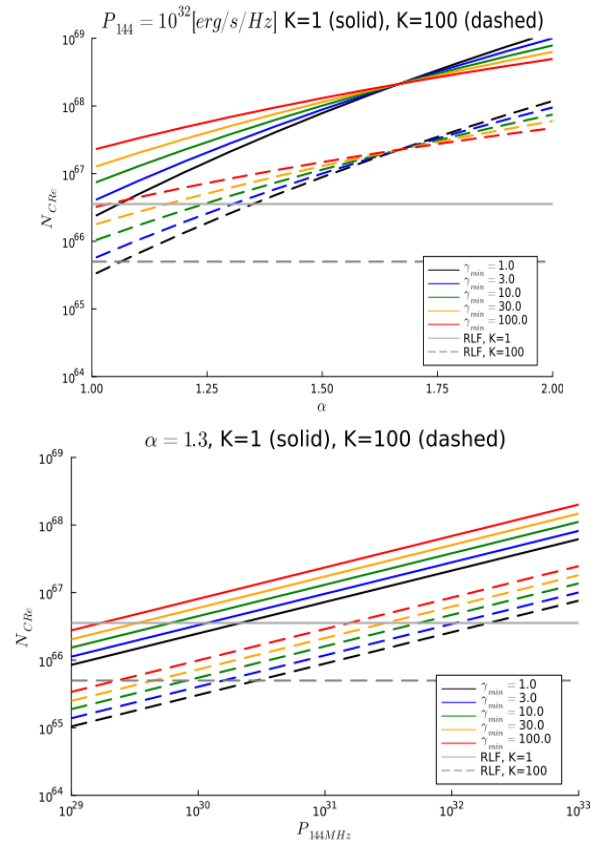
Figure 2. Top panel: number of cosmic ray electrons to explain a radio halo emitting 10^{32} \text{ erg/s/Hz} at 144 MHz, as a function of the observed radio spectrum ( \alpha ) and for different choices of the ratio between cosmic ray protons and electrons ( k ) and for different choices of the minimum energy of electrons. Bottom panel: number of cosmic ray electrons required to explain radio halo emissions of different power at 144 MHz, assuming \alpha = 1.3 , \gamma_{\min} = 10 and for K = 1 or K = 100 . In both panels we assume that the radio halo has a volume of 1^3 \text{ Mpc}^3 and that the host cluster has a 10^{15} M_{\odot} mass. The horizontal lines give the number of electrons injected by the entire population of radio galaxies in a cluster and only using a single activity burst, assuming a \alpha = 0.8 spectrum for all radio galaxies, and either K = 1 or K = 100 .
