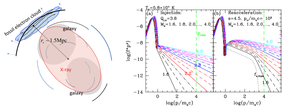
Figure 3. Left: cartoon sketch of the bubble of fossil relativistic electrons at the location of the "Sausage" radio relic in cluster CIZA J2242.8+5301. Right plots: electrons spectra resulting from the injection of fresh electrons via diffusive shock acceleration, as a function of Mach number (central panel), or from the re-acceleration of fossil relativistic electrons by the same shocks. Taken from [116].
