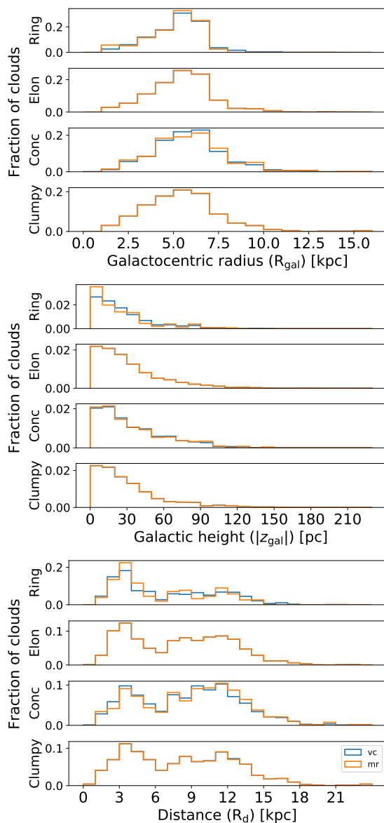
Fig. 6: Histogram (normalised) for distribution of clouds with respect to Galactocentric radius [top] Galactic height ( z_{\text{gal}} ) [middle], and heliocentric distance [bottom]. The histograms represent the ratio of clouds in each bin to the total number of clouds in all the bins. The bin width is 1 kpc for the heliocentric distance and Galactocentric radius plots and 1 pc for the z_{\text{gal}} histogram. The blue colour represents the VC sample and the orange colour represents the morphologically reliable (MR) sample. The cloud morphologies from top to bottom represent ring-like clouds (Ring), elongated clouds (Elon), concentrated clouds (Conc) and clumpy clouds (Clumpy).
