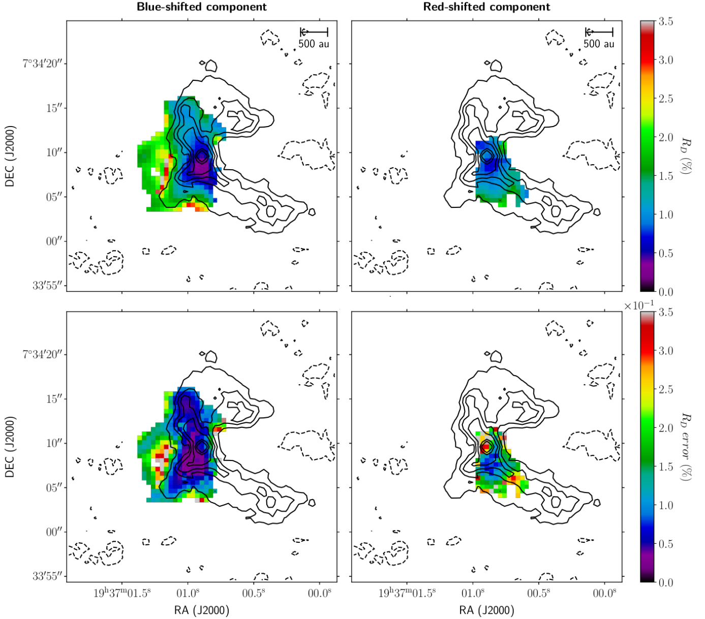
Fig. 2. Dust continuum emission at 110 GHz for -2 , 3 , 5 , 7 , 10 , 30 , and 50\sigma (black contours) superimposed on the deuterium fraction maps ( top panels ) and on the corresponding statistical uncertainties ( lower panels ) for the blue- and redshifted velocity components ( left and right columns , respectively). The spatial scale is shown in the top-right corner of the upper panels .
