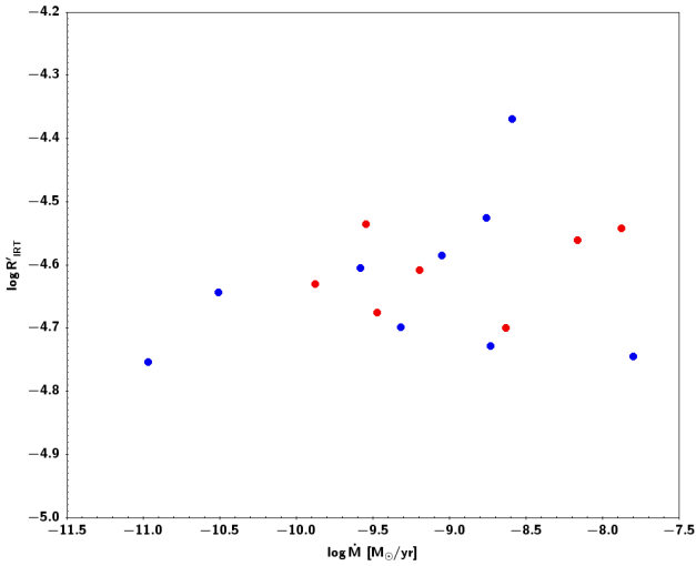
Fig. 8. Activity index ( \log R'_{\text{IRT}} ) vs. accretion rate ( \log \dot{M} ) for selected sources. Red filled circles indicate accretion rates derived from the width of H\alpha at 10% of the peak by the Gaia -ESO survey (Lanzafame et al. 2015, and references therein). Blue filled circles indicate accretion rates derived from the excess continuum emission (see, e.g. Manara et al. 2015). See Table 2 for the sources of the accretion rate estimates.
