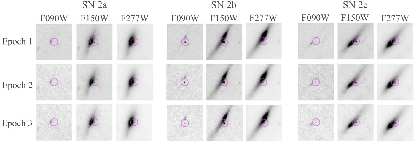
Figure 10. Time series of SN H0pe imaging observations. Negative images in the three epochs are shown for each of the three images of the SN. Of the eight NIRCcam filters acquired in Epoch 1 and six filters in each of Epochs 2 and 3, only three filters are depicted for clarity. The image stamps are oriented north up, east left and are 3'' on a side. The SN appeared first in image 2a, where it was intercepted on the decline after the second IR peak in the light curve. SN 2a and SN 2b were intercepted near the first peak, and Epochs 2 and 3 also trace the second peak detected in the NIRCcam LW channels of this SN Ia.
