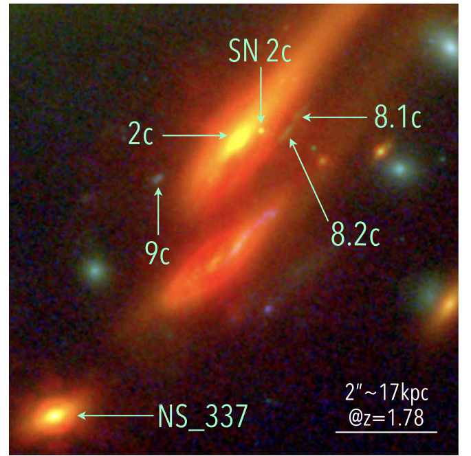
Figure 3. NIRCам color image centered on one of the SN host images 2c (Arc 2c), along with three other galaxies spectroscopically confirmed to be at z = 1.78 in this study. Our lens model predicts for Arcs 2, 8, 9, and NS_337 to be situated within 33 physical kiloparsecs in the source plane. The NIRSpec spectra of these arcs appear in Figure 4. Colors follow the prescription in Trilogy (Coe et al. 2012) with red showing F444W and F356W, green showing F277W and F200W, and blue showing F150W and F090W.
