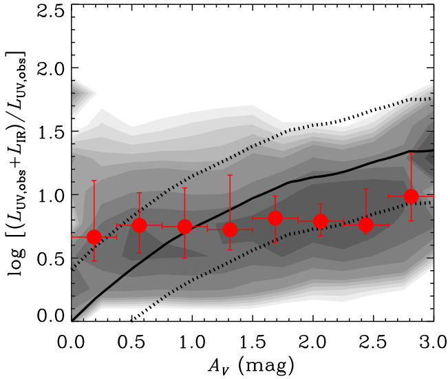
Figure 1. Ratio of observed UV plus IR luminosity to observed UV luminosity ( (L_{\text{UV,obs}} + L_{\text{IR}})/L_{\text{UV,obs}} ) vs. measured V-band attenuation A_V (in magnitudes) for the 931 galaxies with IR detections (smooth contours). The darkest portions of the contours indicate the highest concentration of sources. Median values and 1\sigma intervals of (L_{\text{UV,obs}} + L_{\text{IR}})/L_{\text{UV,obs}} , in bins of A_V , are indicated as filled red circles with error bars. The black solid and dotted curves represent the predicted Calzetti et al. (2000) extinction curve, 3.2/C(A_V)10^{0.72A_V} , and 1\sigma interval ( \approx 0.5 dex), respectively.
