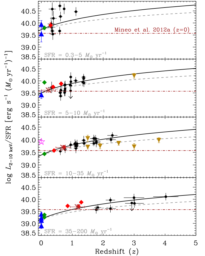
Figure 9. Stacked 2–10 keV luminosity per unit SFR ( L_{2-10 \text{ keV}}/\text{SFR} ) vs. redshift for sSFR-selected galaxy subsamples divided into four SFR intervals. Symbols have the same meaning as in Figure 8, except that the sizes of each symbol are constant. In each panel, the solid curve indicates our best-fit redshift and SFR dependent model, \log L_{2-10 \text{ keV}} = A_3 + B_3 \log \text{SFR} + C_3 \log(1+z) , which was fit to the combined L10 and CDF-S stacked data. For comparison the Mineo et al. (2012a) relation for high-sSFR galaxies has been shown as a brown dashed-dot curve. The curves are plotted using the median SFR of the L10 and CDF-S data points in that panel. The dashed curves show the equivalent relation, derived by Basu-Zych et al. (2013b), using the same functional form but with different stacked data. The redshift-dependence of L_{2-10 \text{ keV}}/\text{SFR} is obvious in each panel and the inclusion of redshift as a model parameter provides a substantive statistical improvement over a constant L_{2-10 \text{ keV}}/\text{SFR} ratio model.
