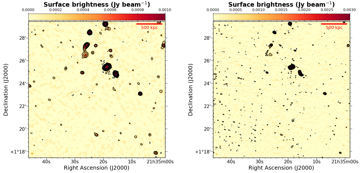
Fig. A.7. Images of the cluster A2355. Left panel: JVLA C array 1.5 GHz image. Contours start at 3\sigma_{\text{rms}} and are spaced by a factor of two. 1\sigma_{\text{rms}} = 0.04 \text{ mJy beam}^{-1} with beam = 11.6'' \times 10.8'' . Right panel: GMRT 610 MHz image. Contours start at 3\sigma_{\text{rms}} and are spaced by a factor of two. 1\sigma_{\text{rms}} = 0.13 \text{ mJy beam}^{-1} with beam = 8.3'' \times 6.1'' .
