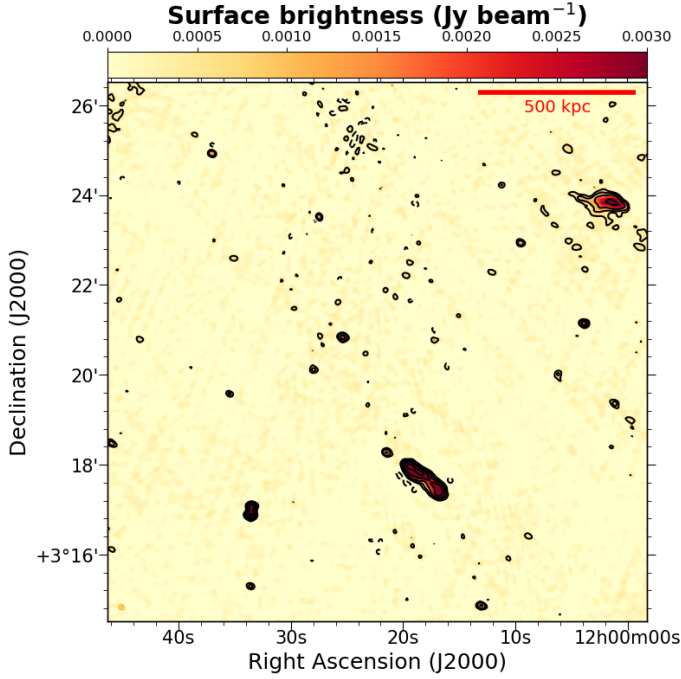
Fig. A.16. A1437 GMRT 330 MHz image. Contours start at 3\sigma_{\text{rms}} and are spaced by a factor of two. 1\sigma_{\text{rms}} = 0.4 \text{ mJy beam}^{-1} with beam = 9.0'' \times 7.4'' .
