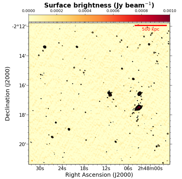
Fig. A.3. Images of the cluster A384. Left panel: JVLA C array 1.5 GHz image. Contours start at 3\sigma_{\text{rms}} and are spaced by a factor of two. 1\sigma_{\text{rms}} = 0.035 \text{ mJy beam}^{-1} with beam = 13.5'' \times 10.4'' . Right panel: GMRT 610 MHz image. Contours start at 3\sigma_{\text{rms}} and are spaced by a factor of two. 1\sigma_{\text{rms}} = 0.05 \text{ mJy beam}^{-1} with beam = 5.9'' \times 4.8'' .
