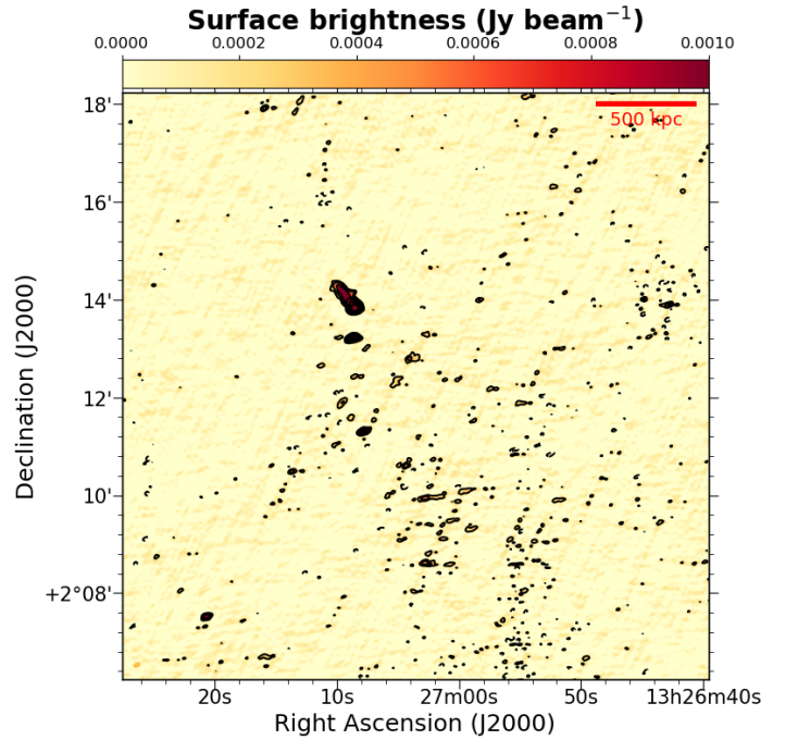
Fig. A.12. A1733 GMRT 610 MHz image. Contours start at 3\sigma_{\text{rms}} and are spaced by a factor of two. 1\sigma_{\text{rms}} = 0.06 \text{ mJy beam}^{-1} with beam = 7.9'' \times 5.0'' .
