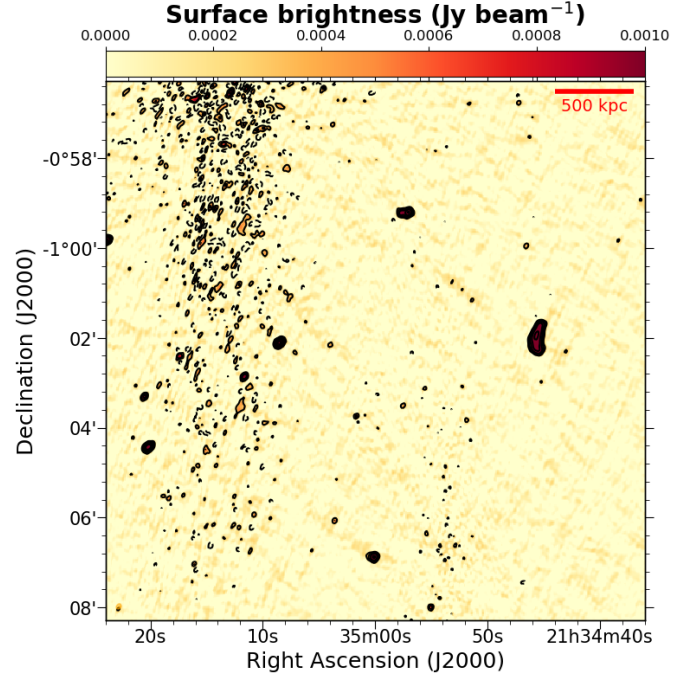
Fig. A.14. MACS J2135-010 GMRT 610 MHz image. Contours start at 3\sigma_{\text{rms}} and are spaced by a factor of two. 1\sigma_{\text{rms}} = 0.08 \text{ mJy beam}^{-1} with beam = 7.8'' \times 5.8'' .
