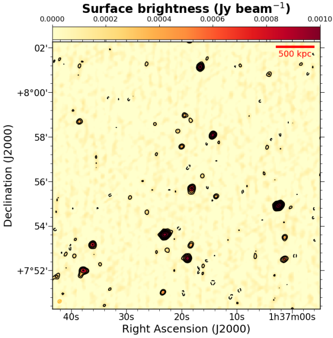
Fig. A.5. A220 JVLA C array 1.5 GHz image. Contours start at 3\sigma_{\text{rms}} and are spaced by a factor of two. 1\sigma_{\text{rms}} = 0.045 \text{ mJy beam}^{-1} with beam = 11.6'' \times 9.8'' .
