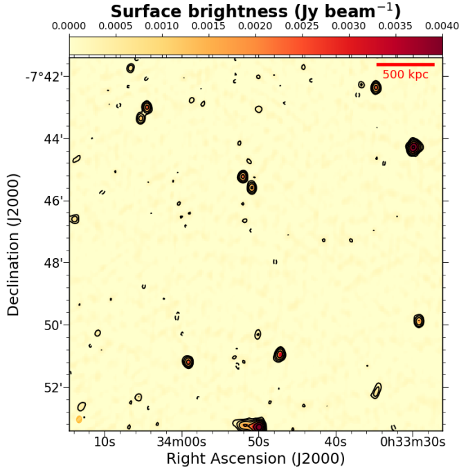
Fig. A.1. A56 JVLA C array 1.5 GHz image. Contours start at 3\sigma_{\text{rms}} and are spaced by a factor of two. 1\sigma_{\text{rms}} = 0.08 \text{ mJy beam}^{-1} with beam = 13.'' \times 10.4'' .
