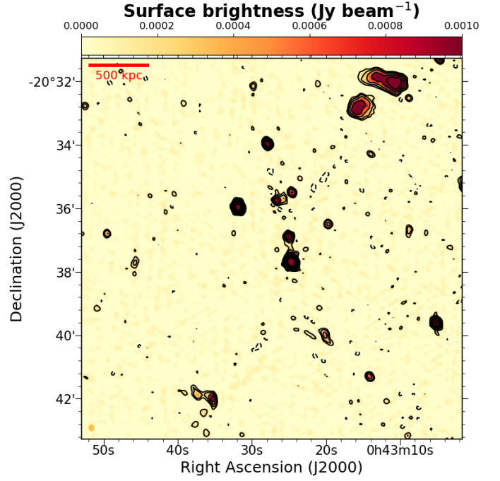
Fig. A.2. A2813 JVLA C array 1.5 GHz image. Contours start at 3\sigma_{\text{rms}} and are spaced by a factor of two. 1\sigma_{\text{rms}} = 0.035 \text{ mJy beam}^{-1} with beam = 11.4'' \times 9.5'' .
