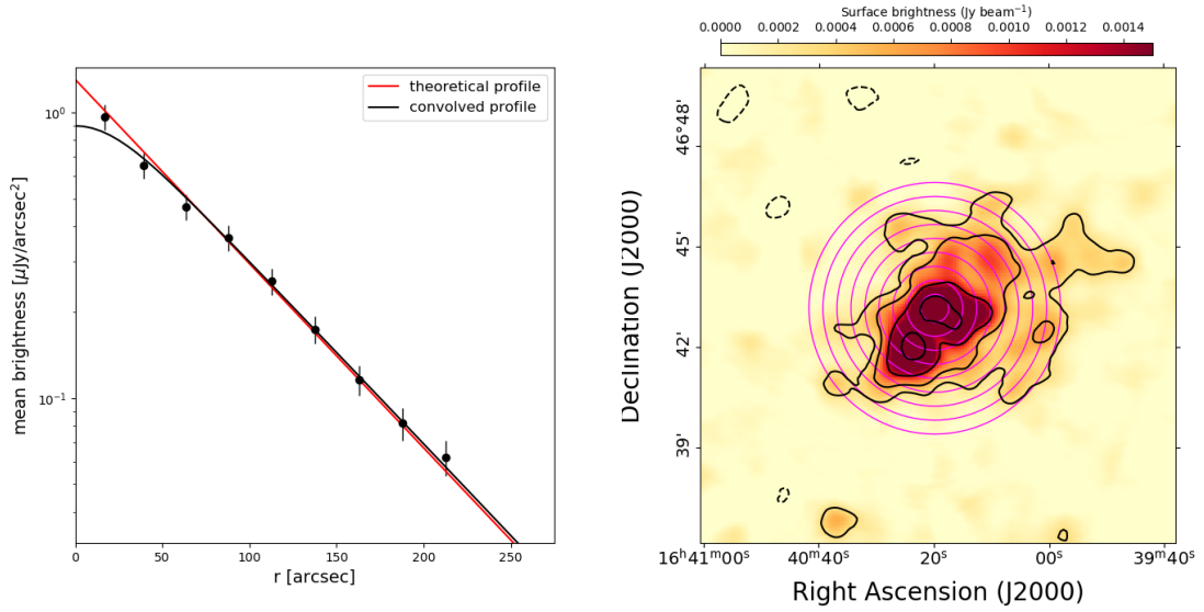
Fig. B.7. Same as Fig. B.1 for A2219.
