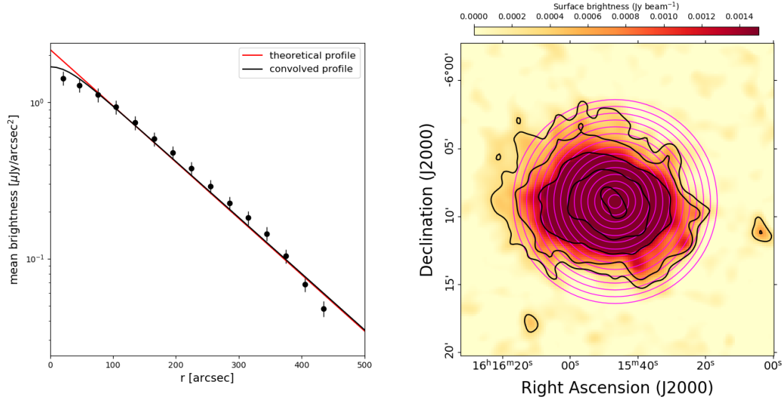
Fig. 10. Radial surface brightness profile of the radio halo in A2163. Left: data points represents the averaged surface brightness measured in the annuli shown in the right panel. The red curve is the theoretical exponential profile, the black curve is the profile convolved with the beam of the image. Right: VLA 1.4 GHz image from where the profile on the left panel has been extracted. The magenta annuli represent the regions where the average surface brightness was measured. Contours start at 3\text{-}\sigma and are spaced by a factor of two. The 1\text{-}\sigma rms noise of the image is 0.1 \text{ mJy beam}^{-1} with beam = 60'' \times 60'' .
