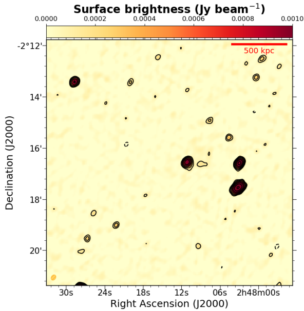
Fig. A.3. Images of the cluster A384. Left panel: JVLA C array 1.5 GHz image. Contours start at 3\sigma_{\text{rms}} and are spaced by a factor of two. 1\sigma_{\text{rms}} = 0.035 \text{ mJy beam}^{-1} with beam = 13.5'' \times 10.4'' . Right panel: GMRT 610 MHz image. Contours start at 3\sigma_{\text{rms}} and are spaced by a factor of two. 1\sigma_{\text{rms}} = 0.05 \text{ mJy beam}^{-1} with beam = 5.9'' \times 4.8'' .
