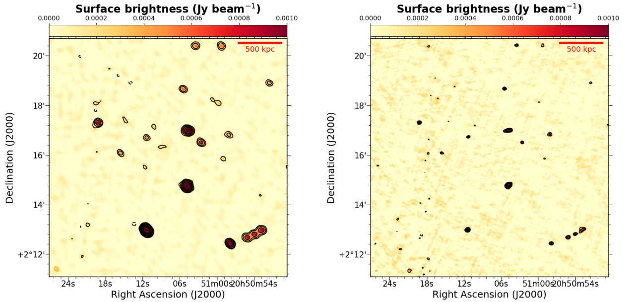
Fig. A.8. Images of the cluster RXC J2051.1+0216. Left panel: JVLA C array 1.5 GHz image. Contours start at 3\sigma_{\text{rms}} and are spaced by a factor of two. 1\sigma_{\text{rms}} = 0.05 \text{ mJy beam}^{-1} with beam = 14.1'' \times 11.5'' . Right panel: GMRT 610 MHz image. Contours start at 3\sigma_{\text{rms}} and are spaced by a factor of two. 1\sigma_{\text{rms}} = 0.1 \text{ mJy beam}^{-1} with beam = 6.0'' \times 4.8'' .
