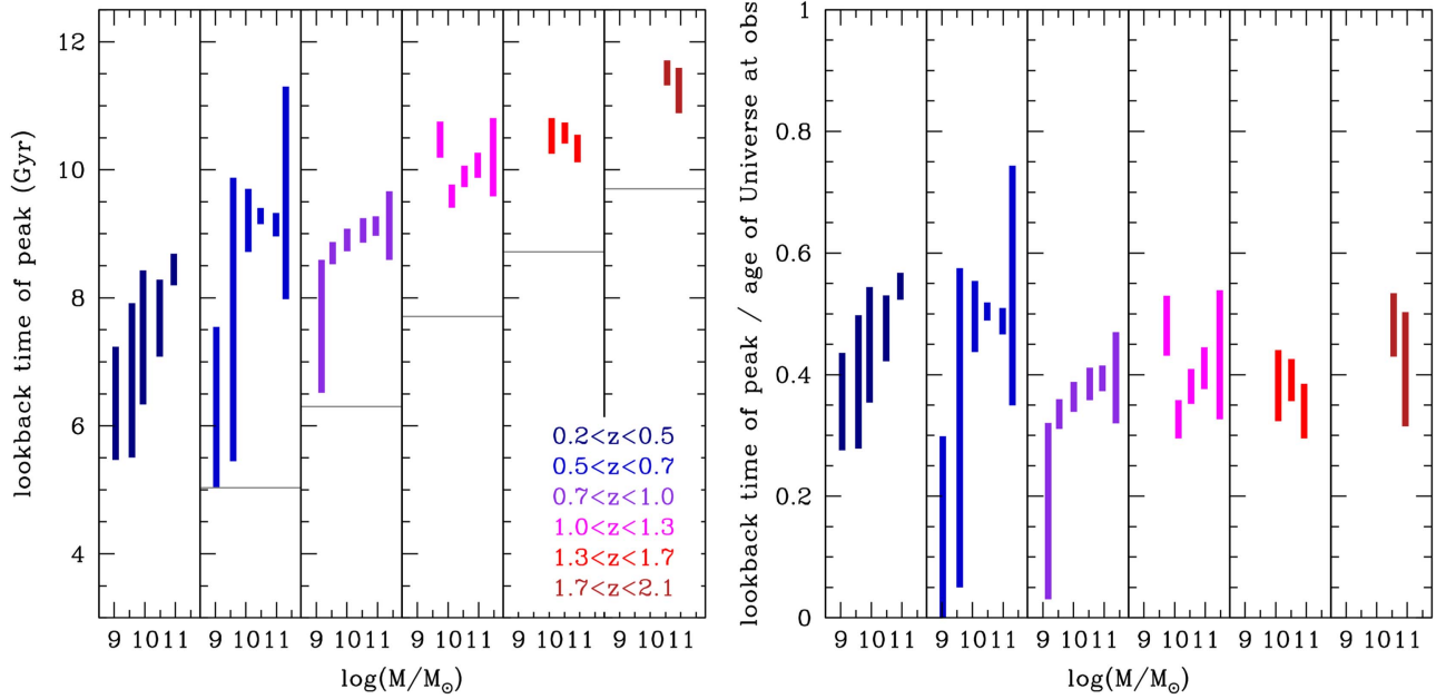
Figure 7. Time at which galaxies reach the peak of their SFHs (vertical lines in Figure 5) is a function of their stellar mass and redshift. Each small panel represents a different redshift bin. Bars are color coded according to redshift. The horizontal gray lines mark the lookback time corresponding to the median redshift of observation of each bin (in the leftmost panel, the gray line is at 2.4 Gyr, thus below the y-axis limit). On the right-hand side, we normalize the lookback time of the peak to the age of the universe at the redshifts of observation.
