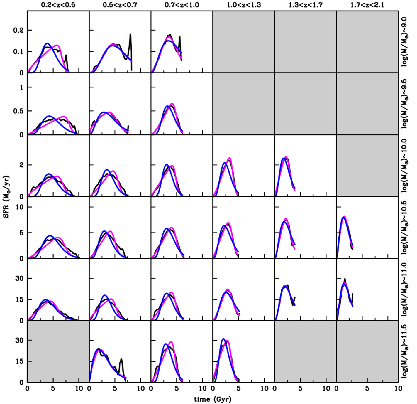
Figure 10. Fits with analytic functions to the median SFHs of Figure 5 (black). Time traces the age of the universe here, and thus it runs in the opposite direction to the lookback time. In blue, a combination of a power law and an exponentially declining function. In magenta, a double power law.
