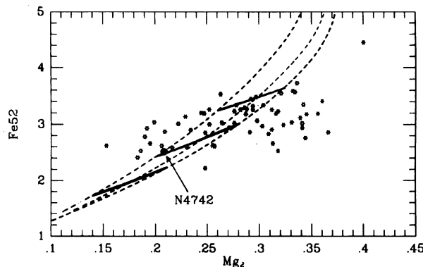
FIG. 17. Evolutionary sequences from 5 to 15 Gyr for three stellar populations with [Fe/H] = -0.5, 0.0, +0.5 (thick solid lines from bottom to top, respectively). Age increases in the sense of increasing Mg_2 . Short-dashed curves are envelopes at 5, 10, and 15 Gyr with changing metallicity. Point markers as in Fig. 16. The galaxy NGC 4742 is singled out (see the text for discussion).
