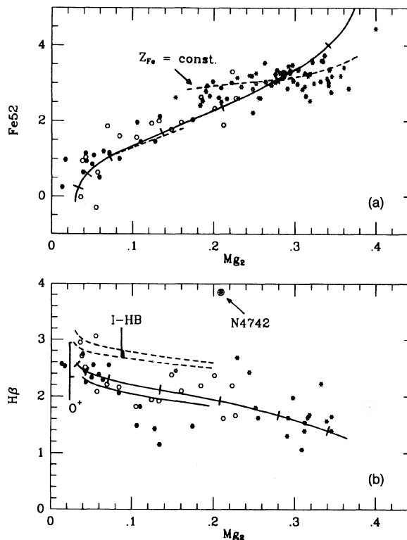
FIG. 16. (a),(b) Adopted metallicity calibration in the observational planes Fe52/Mg_2 and H\beta/Mg_2 . Full and open dots are Galactic and M31 globular clusters from Burstein et al. (1984), while star and asterisk markers are for elliptical galaxies from Gorgas et al. (1990), and Worthey et al. (1992), respectively. Solid curves in both panels indicate the locus expected for standard 15 Gyr Salpeter SSP with RHB. Increasing values for [Fe/H] from -2.5 to +0.5 are marked along the curve every 0.5 dex in the sense of increasing Mg_2 . The effect of adopting an IHB morphology at low metallicities (i.e., for Mg_2 \geq 0.2 ) is displayed in both panels by the dashed lines, while in panel b also the effect of O-enhanced models is accounted for (labels O + ). The Fe52 distribution for galaxies in panel a is better matched if the direct dependence of the index on stellar metallicity in the fitting functions [Eqs. (1)–(3)] is neglected (dashed curve about Mg_2 \sim 0.28 ). See the text for discussion.
