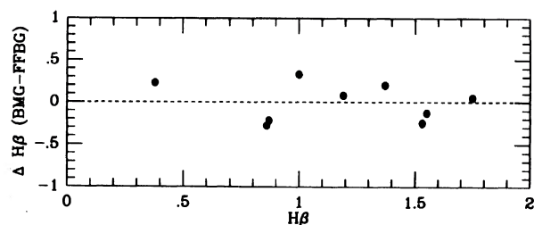
FIG. 8. Calibration residuals of H\beta for the nine standard stars in common with Faber et al. (1985). The standard system is reproduced within \sigma_{H\beta} = \pm 0.23 Å.
