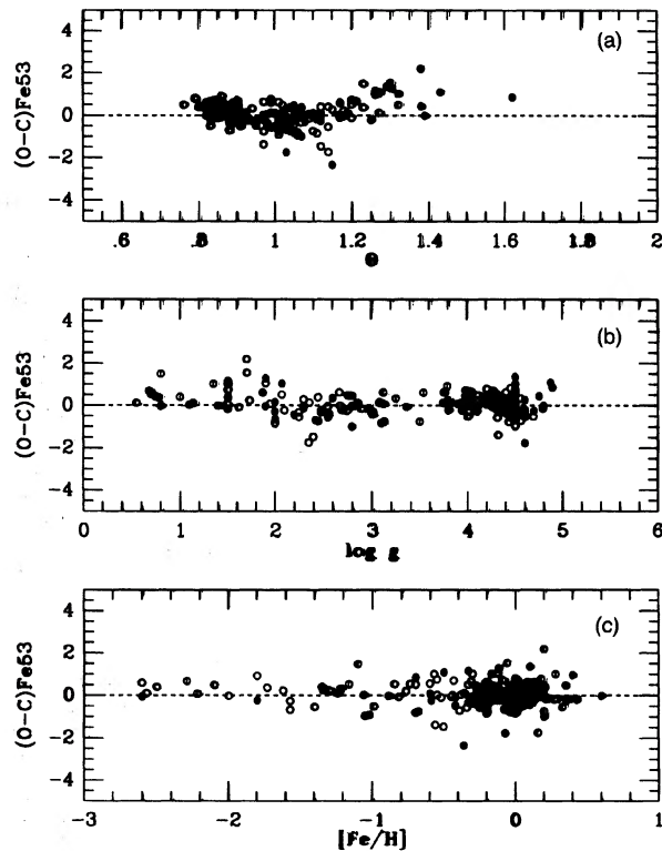
FIG. 5. (a)–(c) Residuals of Fe53 from adopted calibration. Points have the same meaning as in Fig. 3. The scatter is \pm 0.52 Å in our working sample and \pm 0.58 Å for the global sample of 204 points.
