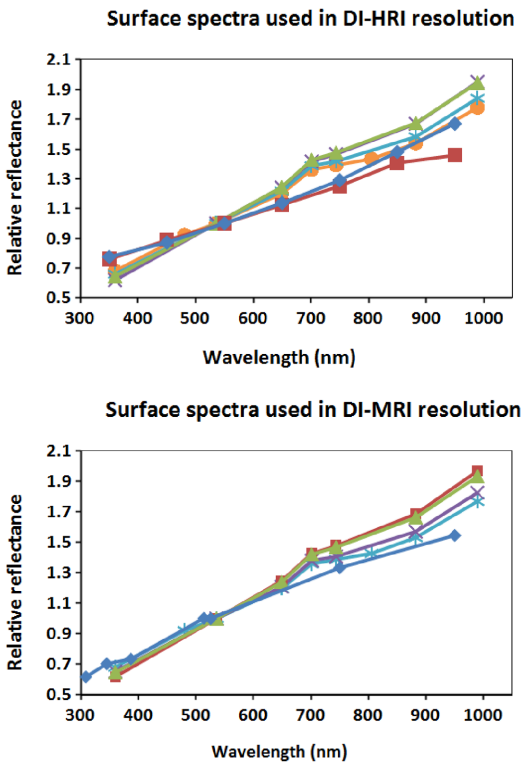
Figure B3. Mean surface spectra considered in this study. Top panel shows the mean surface spectra used in the right-hand column of Fig. 4 and in the top panel of Fig. 7, while the bottom panel shows the mean surface spectra used in the right-hand column of Fig. 5 and in the bottom panel of Fig. 4.
