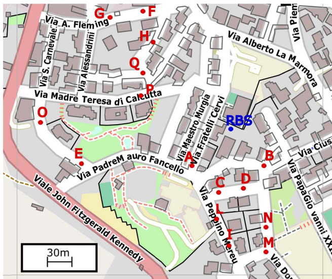
Fig. 8. Geometry of Dorgali measurement campaign at 944.2 MHz. Both the RBS position and the measurement points are shown. The RBS height is 20 m and its pointing direction is 300^\circ .
