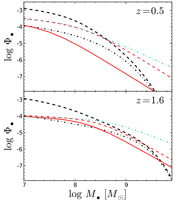
Figure 25. Comparison of our active BHMF with the semi-empirical models of BH growth from Shankar et al. (2013) at two characteristic redshifts, z = 0.5 and 1.6 . The black lines show our results for the obscuration corrected AGN population (dashed) and for type-1 AGN only (dash-dotted). The red and cyan lines present different models from Shankar et al. (2013) always assuming a log-normal ERDF. They tested models with a constant ERDF (red solid line), but also included a z dependence (red dashed line) and an additional M_\bullet dependence (cyan dash-dotted line).
