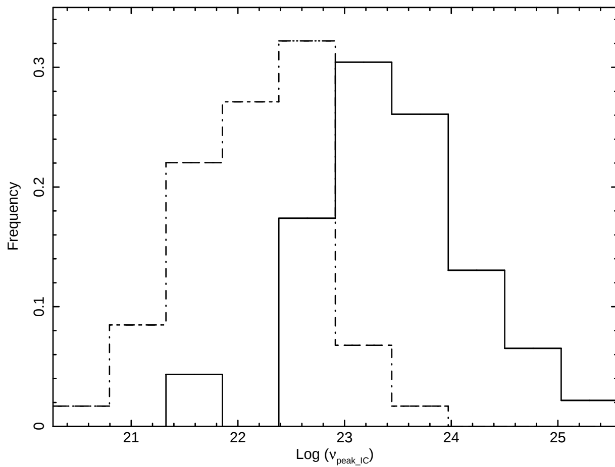
Fig. 33.— The distribution of inverse Compton peak frequency for the sample of LBAS FSRQ (dot-dashed line) and BL Lacs (solid line).
