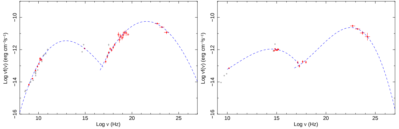
Fig. 24.— The SED of 0FGL J2327.3+0947 = PKS 2325+093 (left) and of 0FGL J2344.5-1559 = PMN J2345-1555 (right)
