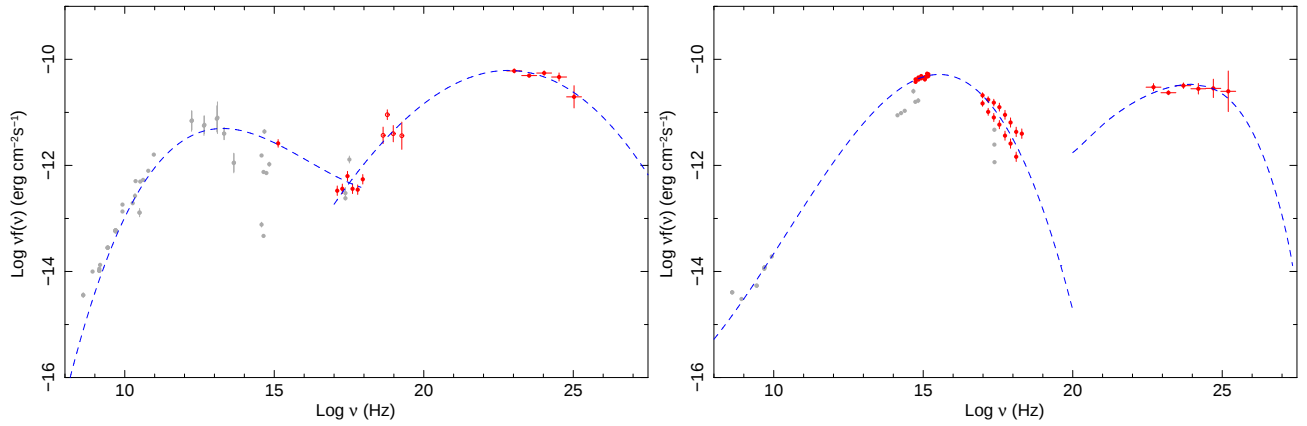
Fig. 6.— The SED of 0FGL J0428.7-3755 = PKS0426-380 (left) and of 0FGL J0449.7-4348 = PKS0447-439 (right)
