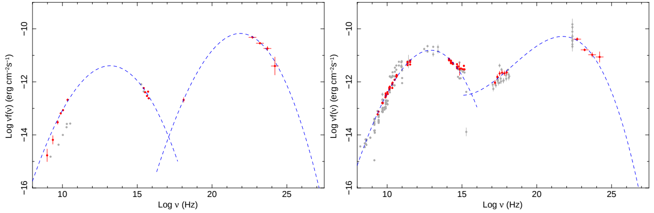
Fig. 5.— The SED of 0FGL J0349.8-2102 = PKS 0347-211 (left) and of 0FGL J0423.1-0112 = PKS0420-01 (right)
