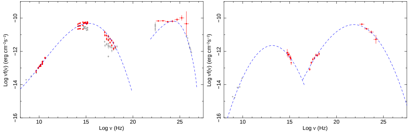
Fig. 3.— The SED of 0FGL J0222.6+4302 = 3C 66A (left) and of 0FGL J0229.5-3640 = PKS0227-369 (right)
