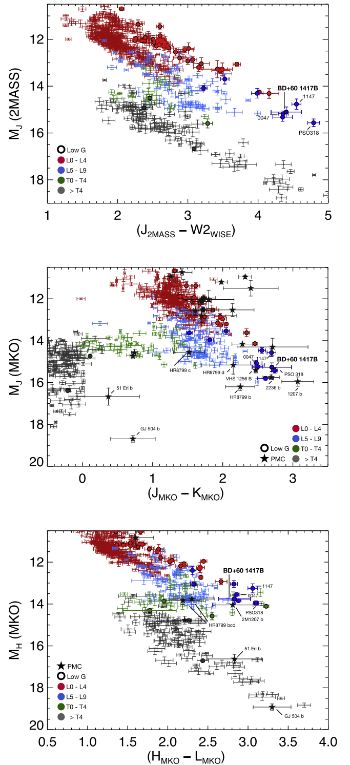
Figure 5. The color–magnitude diagrams for field sources, low-gravity brown dwarfs and directly imaged planetary mass companions color coded by spectral subtype. Top: M_J (2MASS) vs. ( J – W2 ). Middle: M_J (MKO) vs. ( J – K ) (MKO). Bottom: M_H (MKO) vs. ( H – L ) (MKO). In the absence of L -band photometry for brown dwarfs we used the relation in Faherty et al. (2016) to convert WISE W1 photometry to L (MKO).
