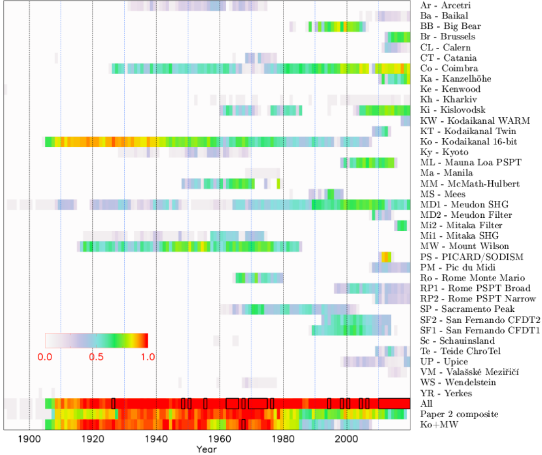
Figure 2. Annual coverage of the various Ca II K archives analysed in this study, except from those taken off-band (see Sect. 2 for details). A color bar in the bottom left corner shows the annual coverage of all the archives combined, the one for the Chatzistergos et al. (2019b, Paper II) composite series, and the annual coverage when only Ko and MW are considered. The annual coverage is colour-coded as shown by the colour bar plotted in the bottom left corner panel. Years with full coverage are outlined with black rectangles.
