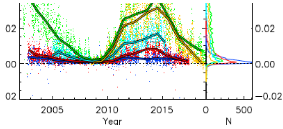
Left: difference of fractional plate area between those derived centred and off-centred Ca II K observations as a function of the differences shown are for the Co-CoW (orange), MD1-MDV (blue), MD1-MDR (red), ML-MLW (cyan). Dots are daily values, while the solid lines show annual median values. A horizontal line denotes a difference of 0. Right: distributions of these differences.
