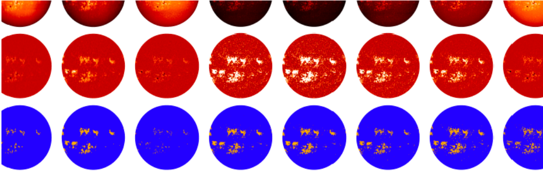
Fig. 12. Examples of observations taken on the same date (04 July 2014) from the various datasets analysed in this study with images not centred on the Ca II K line along with those from the same observatories centred at the core of the Ca II K line. Shown are images from CoW, MDW, MDV, MD1, MDR, ML, MLW datasets after the preprocessing to identify the disc and re-sample them to account for the solar north pole at the top. The raw images are shown to their entire range of values, the CLV-compensated images are shown to the range [-0.5, 0.5] , while in the masks, the plage regions are shown in orange and the quiet Sun and network regions in blue. We stress that the same mask was used for all datasets to identify the plage regions, which is why the different datasets seem to provide rather different ranges of values.
