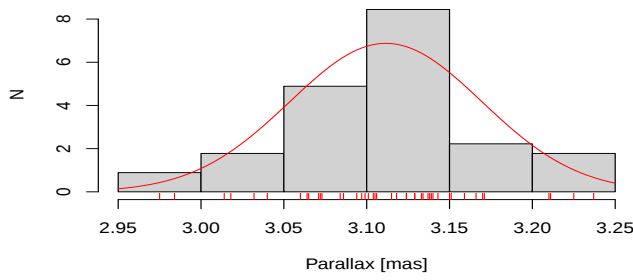
Fig. B.54. Parallax distribution for NGC 2232.
