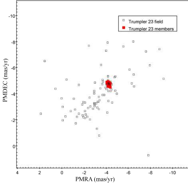
Fig. B.169. PMs diagram for Trumpler 23.
