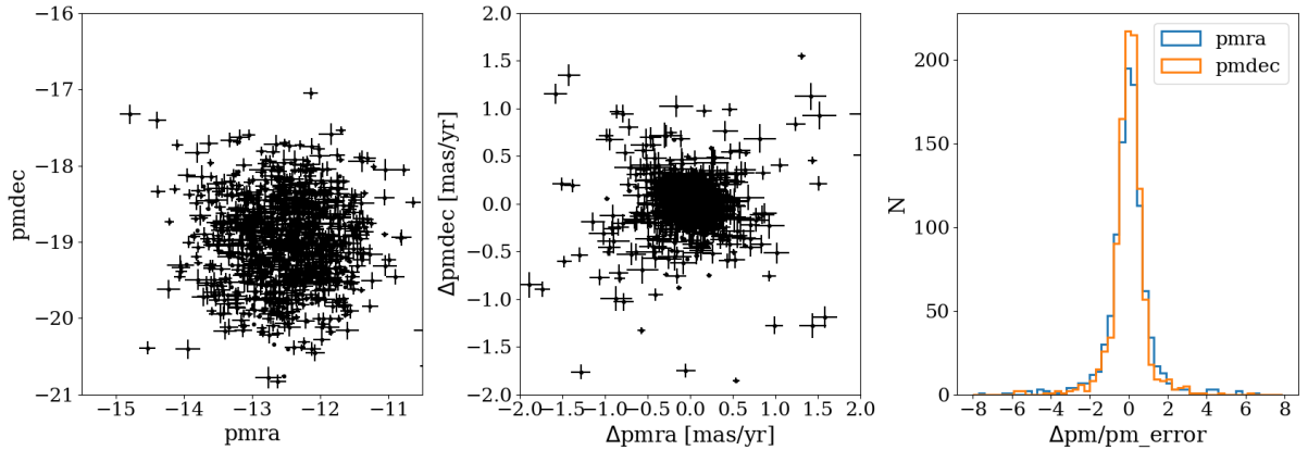
Fig. 26. Left: Gaia proper motion distribution in M4. Only stars with a proper motion error < 0.2 mas yr ^{-1} and flux excess parameter C < 2 are plotted. Centre: Differences between proper motions in Gaia and in HST data. Right: Scaled dispersion for the stars having Gaia proper motions errors < 0.2 mas yr ^{-1} and flux excess parameter C < 2 .
