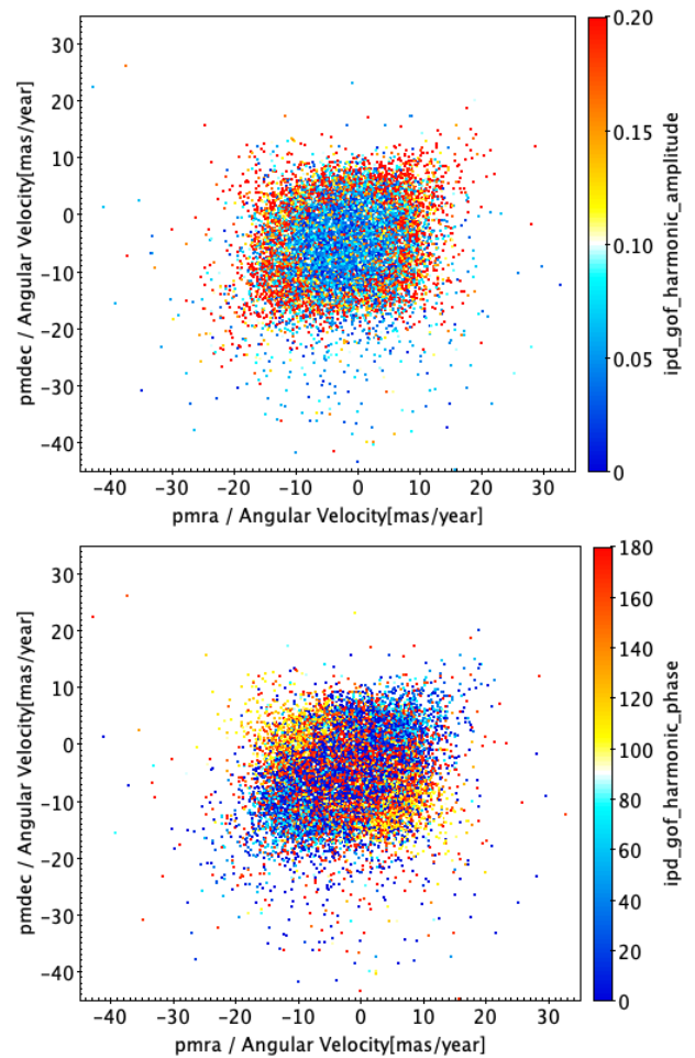
Fig. 14. Proper motion diagram of sources near the Galactic centre within a 0.5^\circ radius. Top: Colour-coded by ipd_gof_harmonic_amplitude . Bottom: Coded by ipd_gof_harmonic_phase . Reddish points in the top panel reveal potentially spurious solutions.
